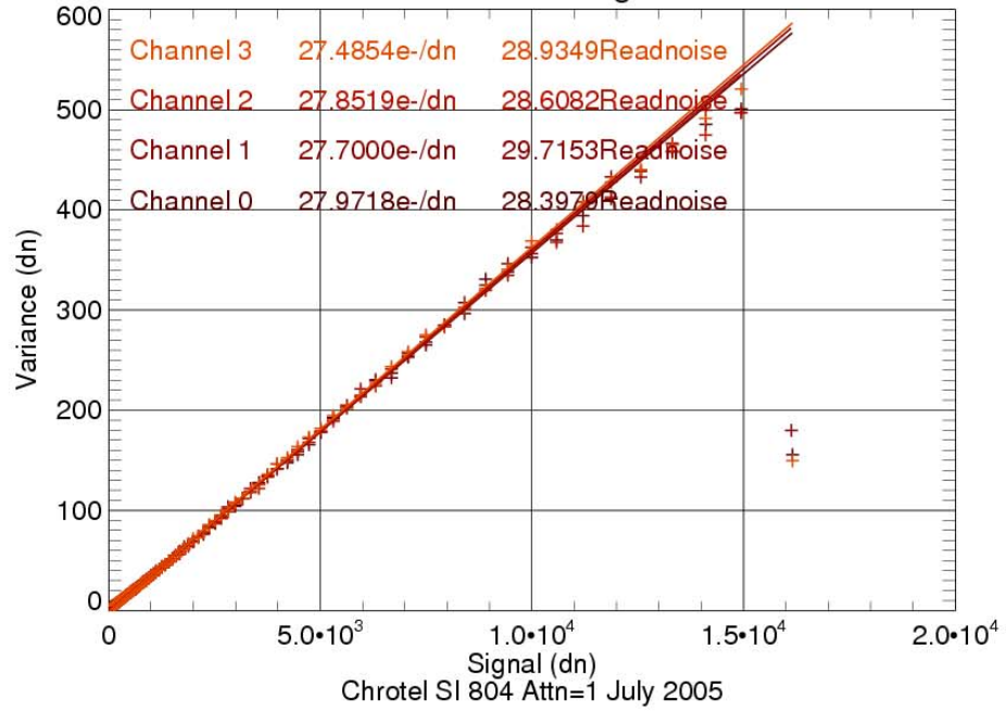
Variance vs. Signal
