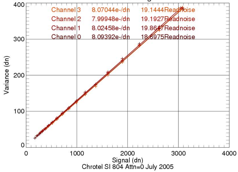
Variance vs. Signal
