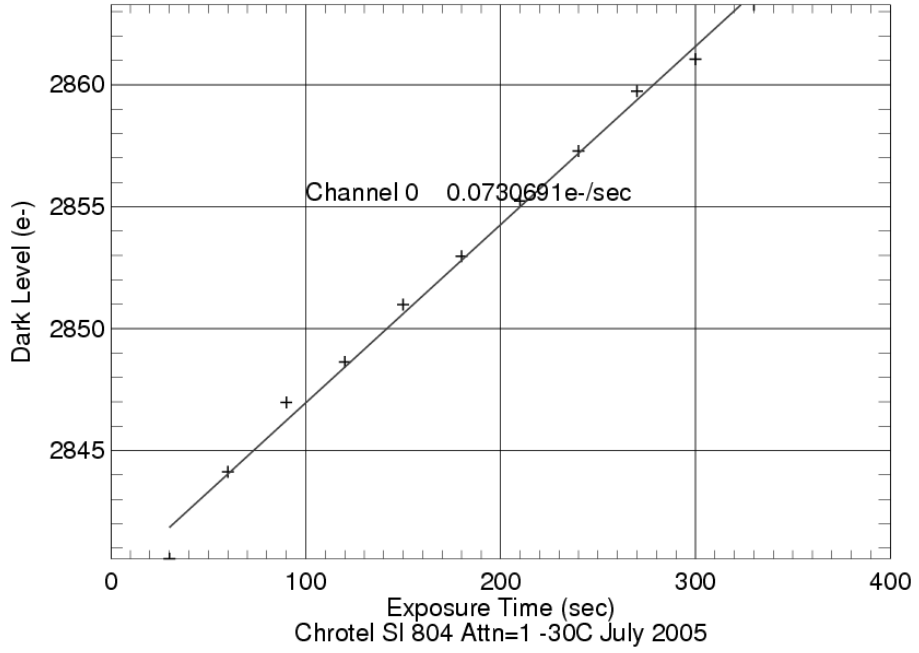
Dark Level vs. Exposure Time
