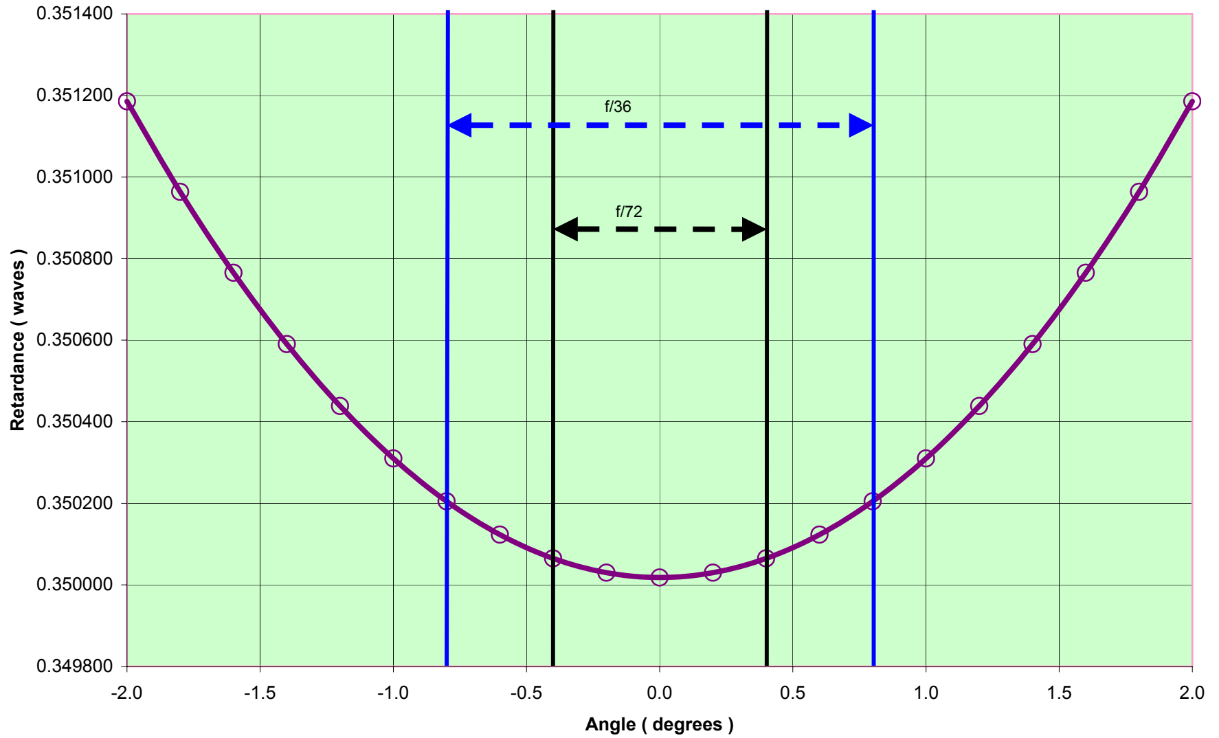
Retardance vs. Angle @ 525nm
