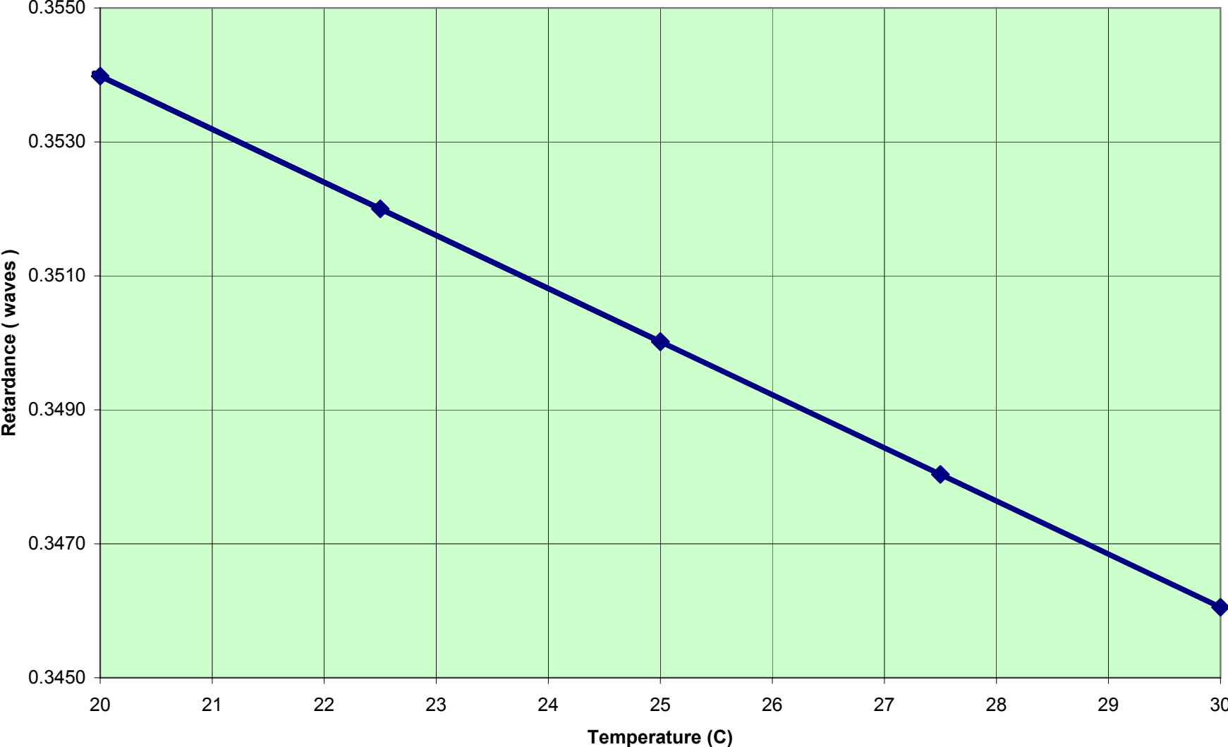
Retardance vs. Temperature @525nm
