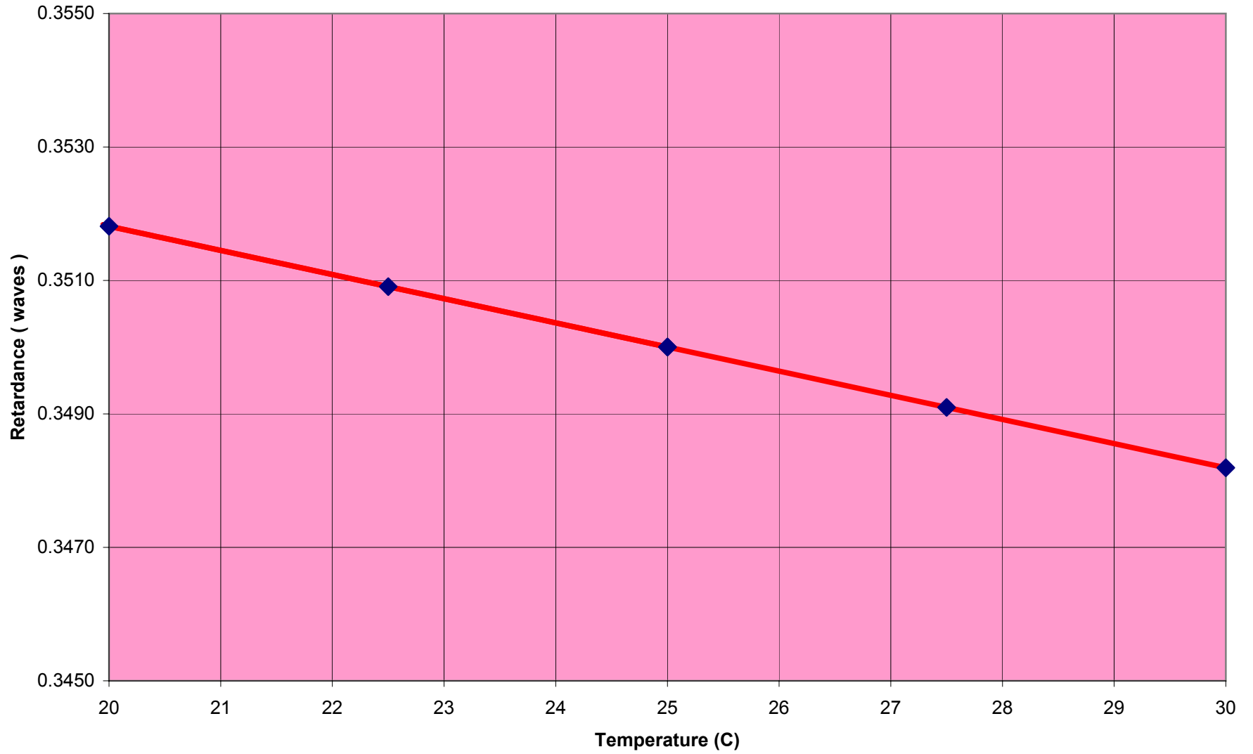
Retardance vs. Temperature @1150nm
